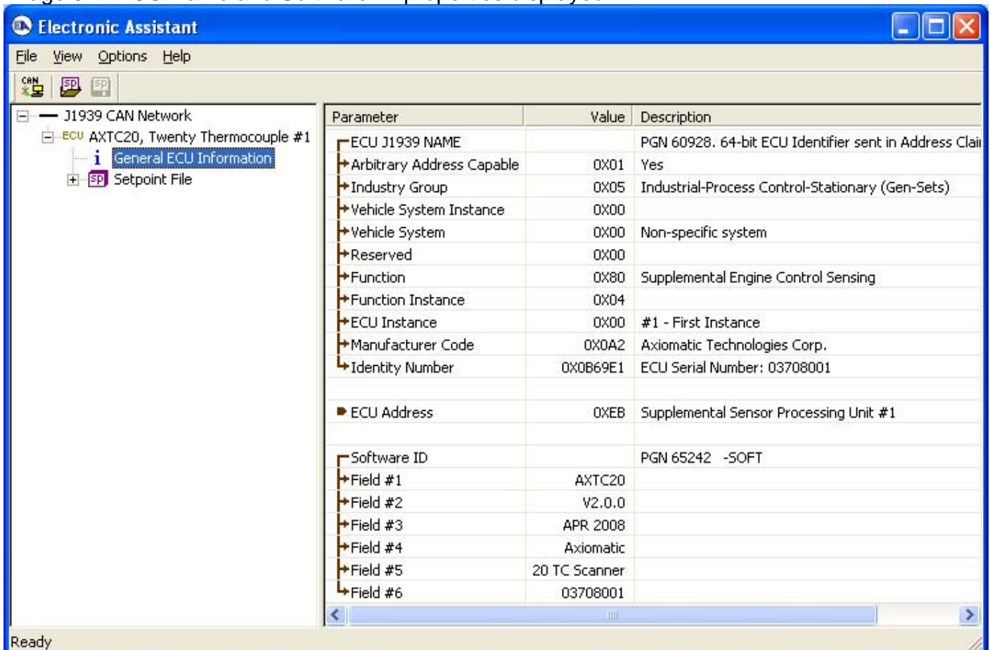
Image 5.2: ECU Name and Software ID properties displayed
