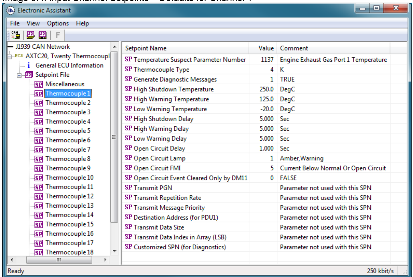
Image 5.4: Input Channel Setpoints – Defaults for Channel 1
