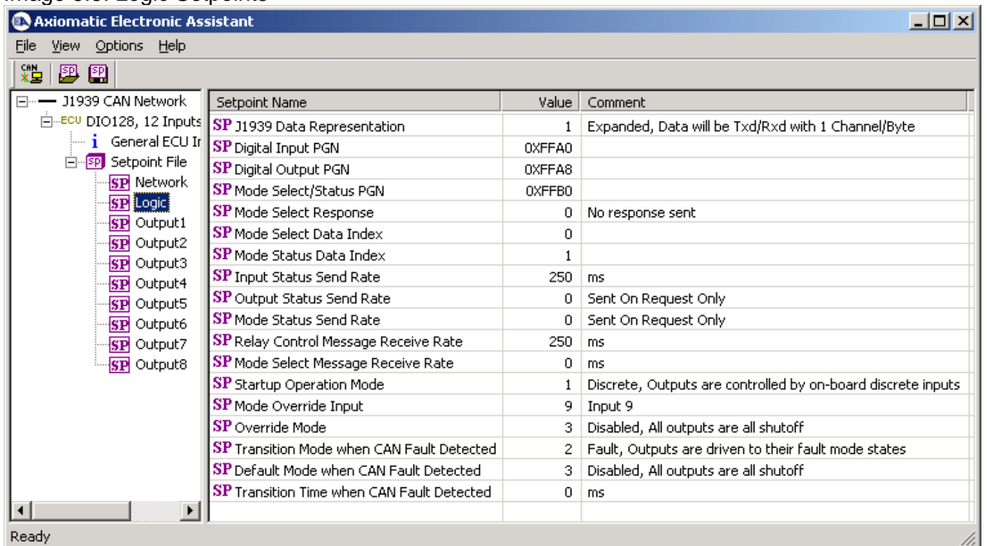
Image 5.5: Logic Setpoints
