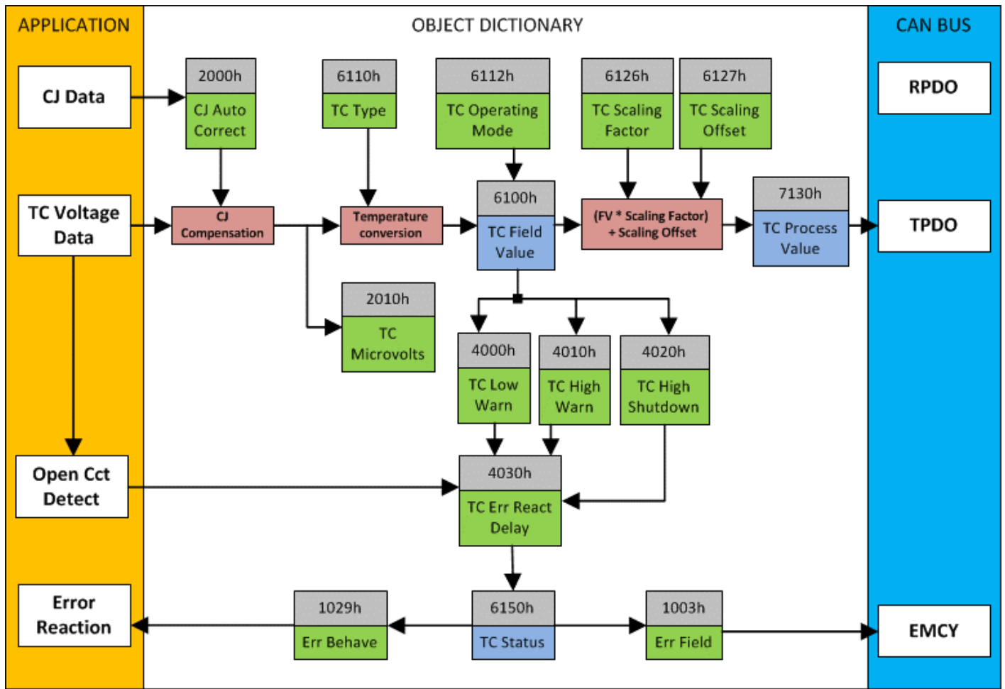
Figure 2 – Thermocouple Input Function Block diagram
