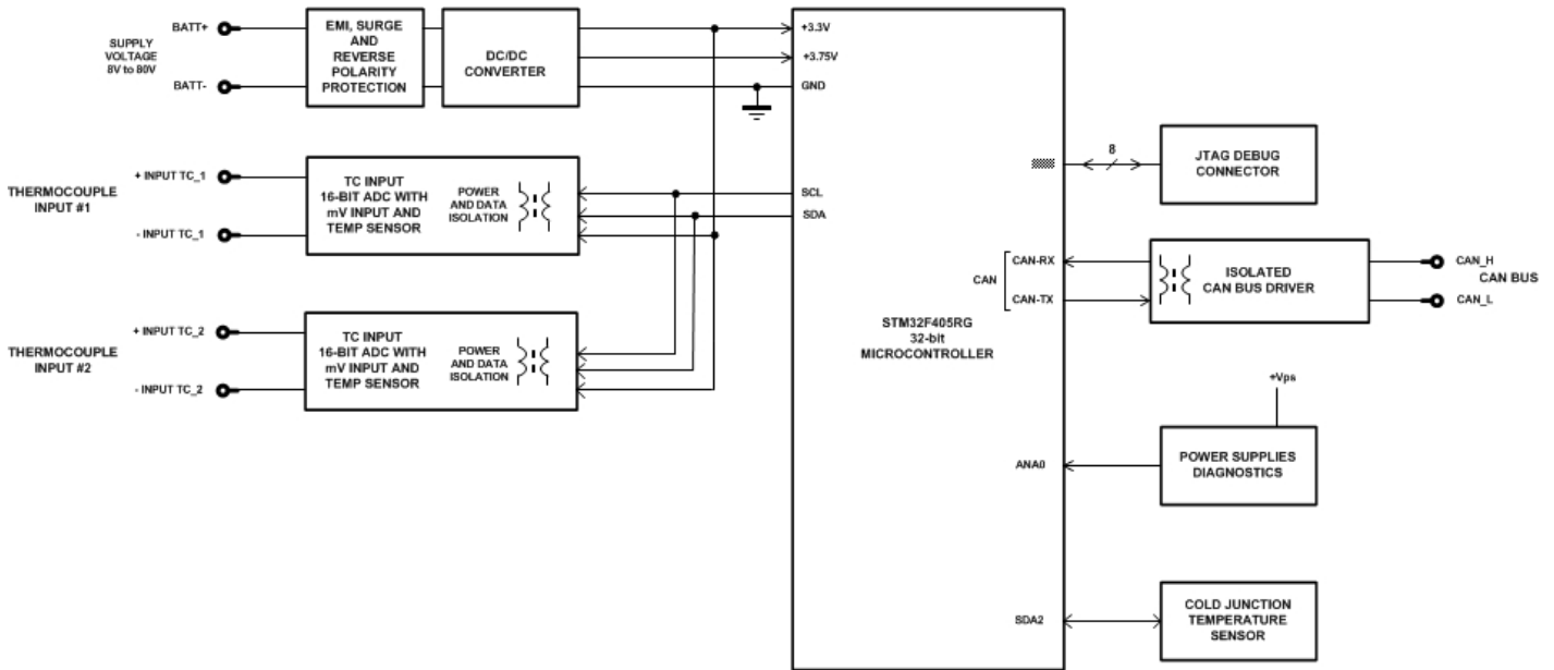
Figure 1 - AX18801 Block Diagram
