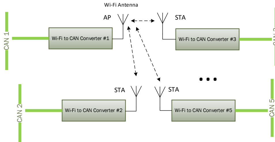
Figure 25. Wireless CAN Bridge with AP/STA Configuration
