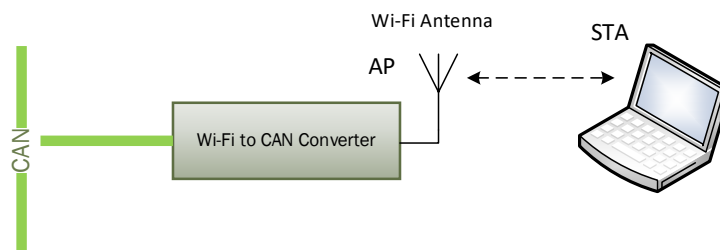
Figure 26. Wireless CAN Access Point
