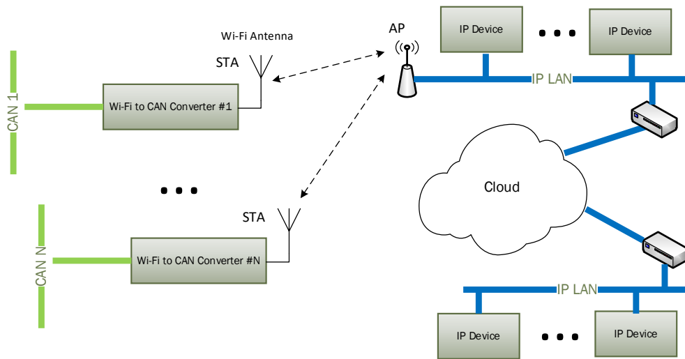
Figure 27. Wireless CAN Station
