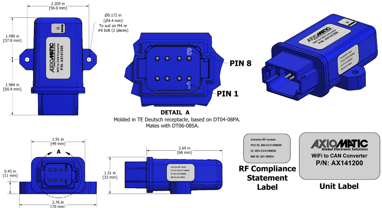
Figure 32. Dimensional Drawing
