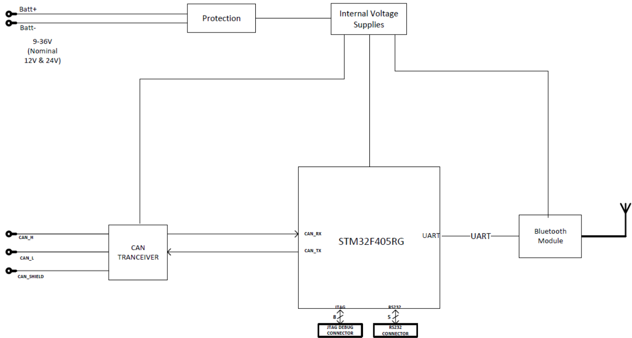
Figure 1 – AX141155 Block Diagram
