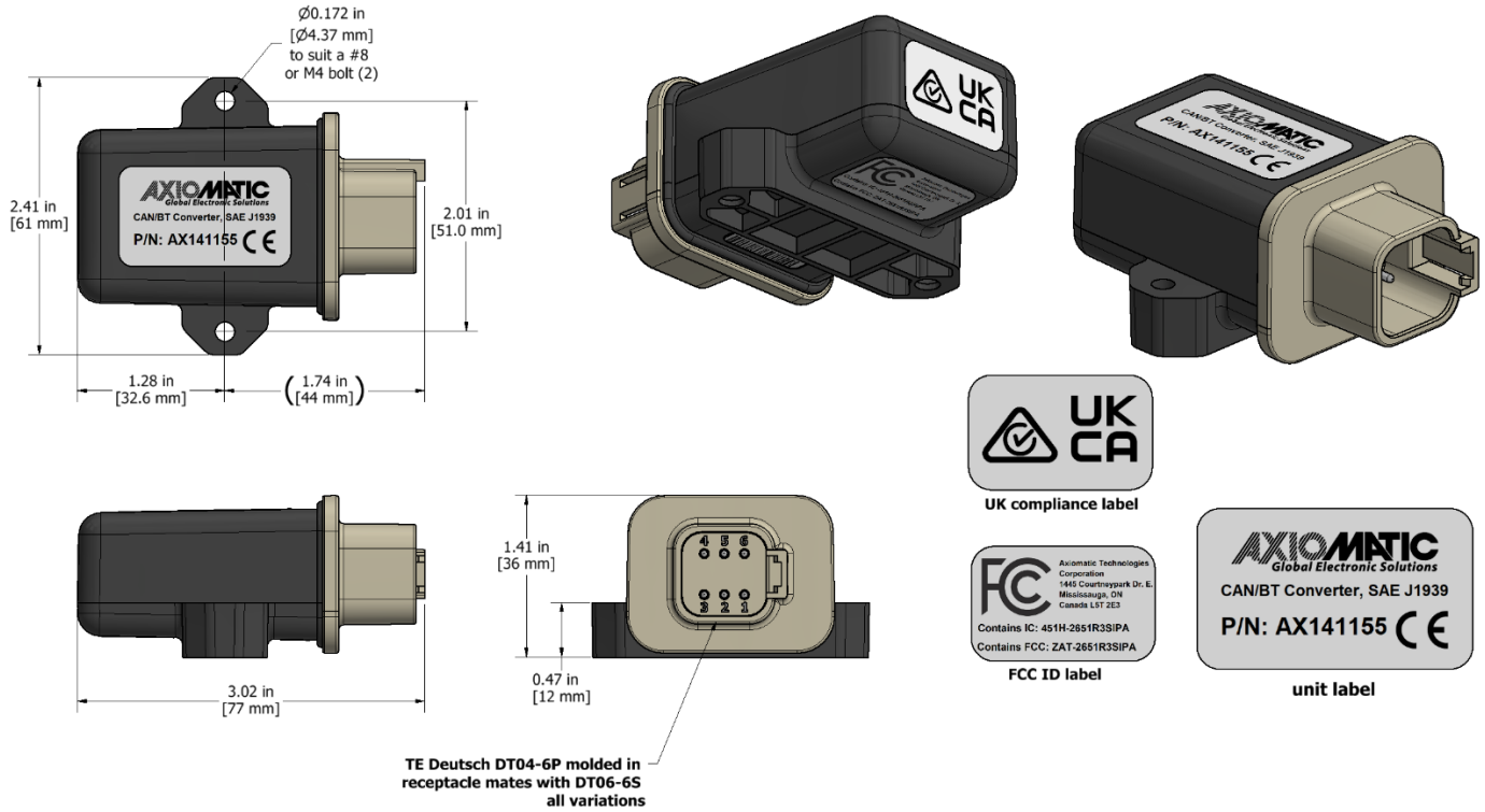
Figure 10 – AX141155 Dimensional Drawing
