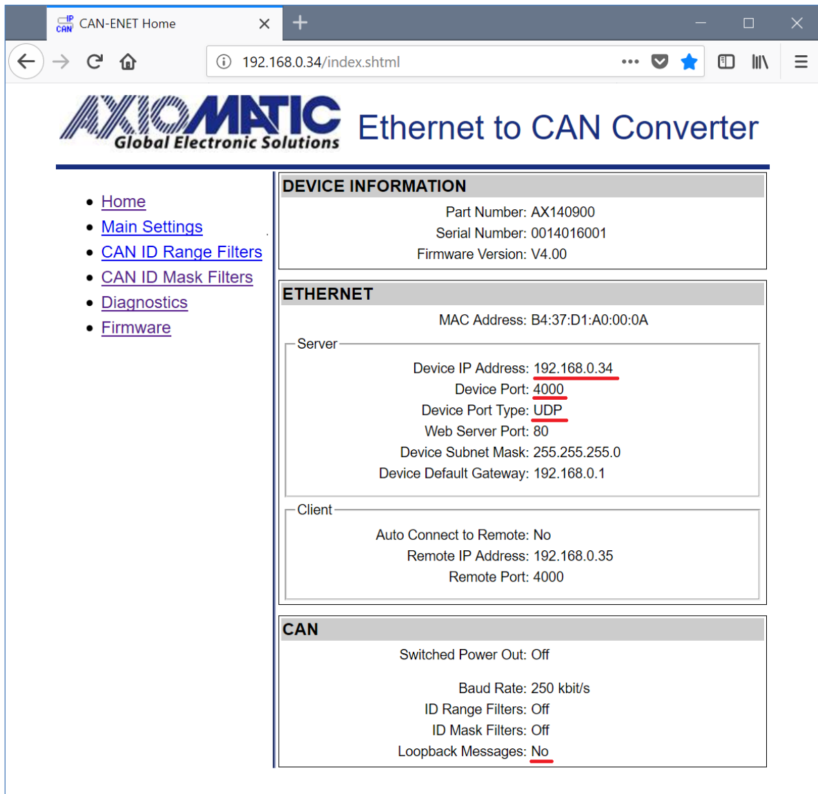
Figure 23. The Converter Server Configuration Example
