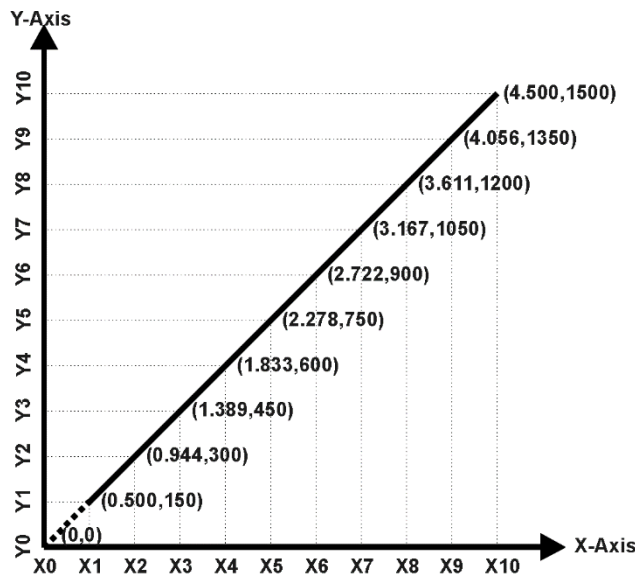
Figure 1 – Lookup Table with “Ramp To” Data Response
