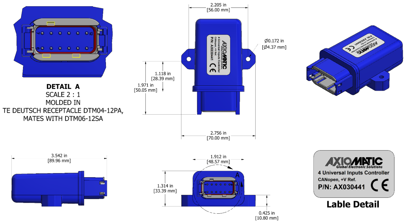
Figure 13 – AX030441 Dimensional Drawing
