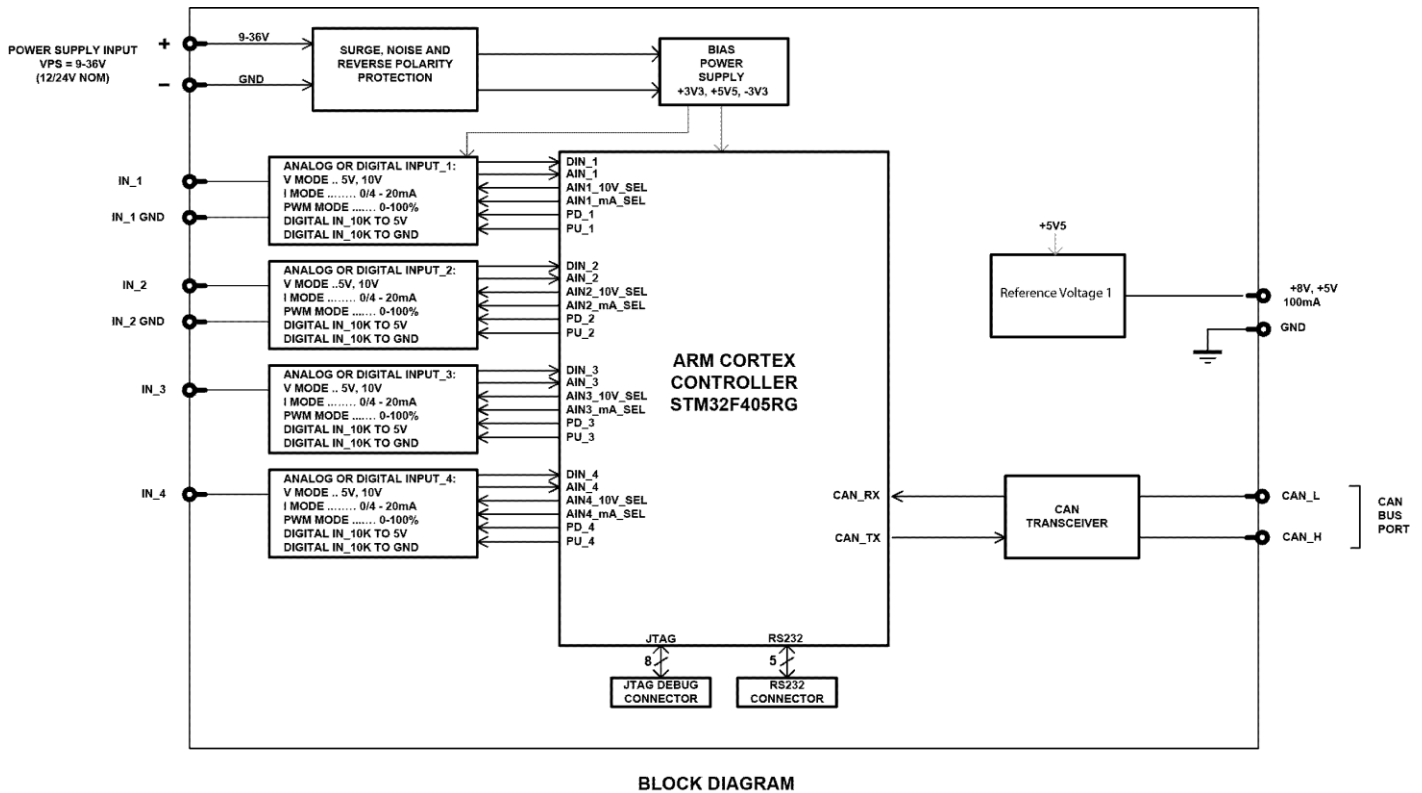
Figure 1 – AX030441 Block Diagram
