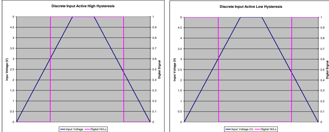
Figure 3 – Discrete Input Hysteresis
