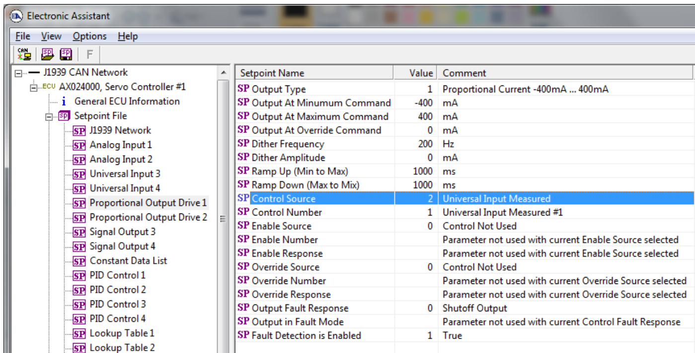
Figure 8 - Screen Capture of Proportional Output Setpoints
