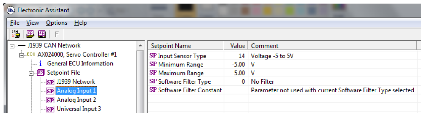
Figure 7 - Screen Capture of Analog Input Setpoints
