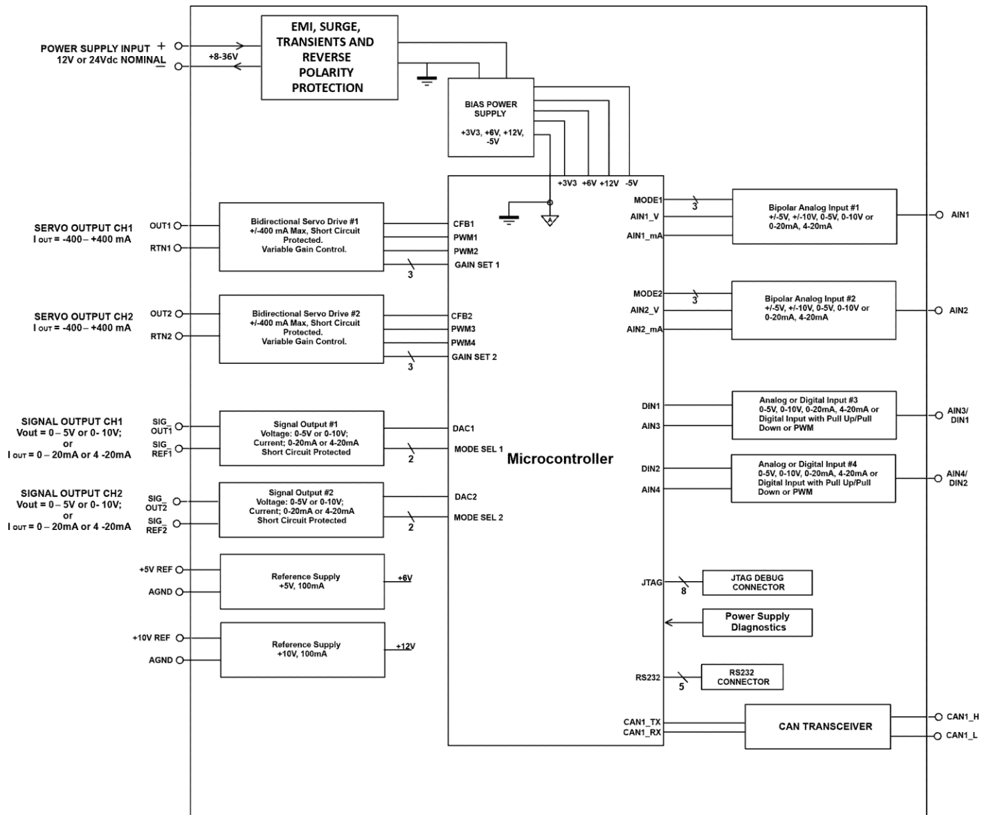
Figure 1 - AX024000 Block Diagram
