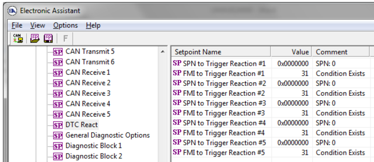
Figure 16 - Screen Capture of DTC React Setpoints
