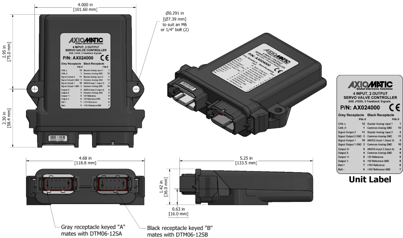
Figure 4 – AX024000 Dimensional Drawing
