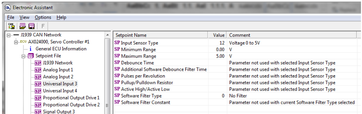
Figure 6 - Screen Capture of Universal Input Setpoints
