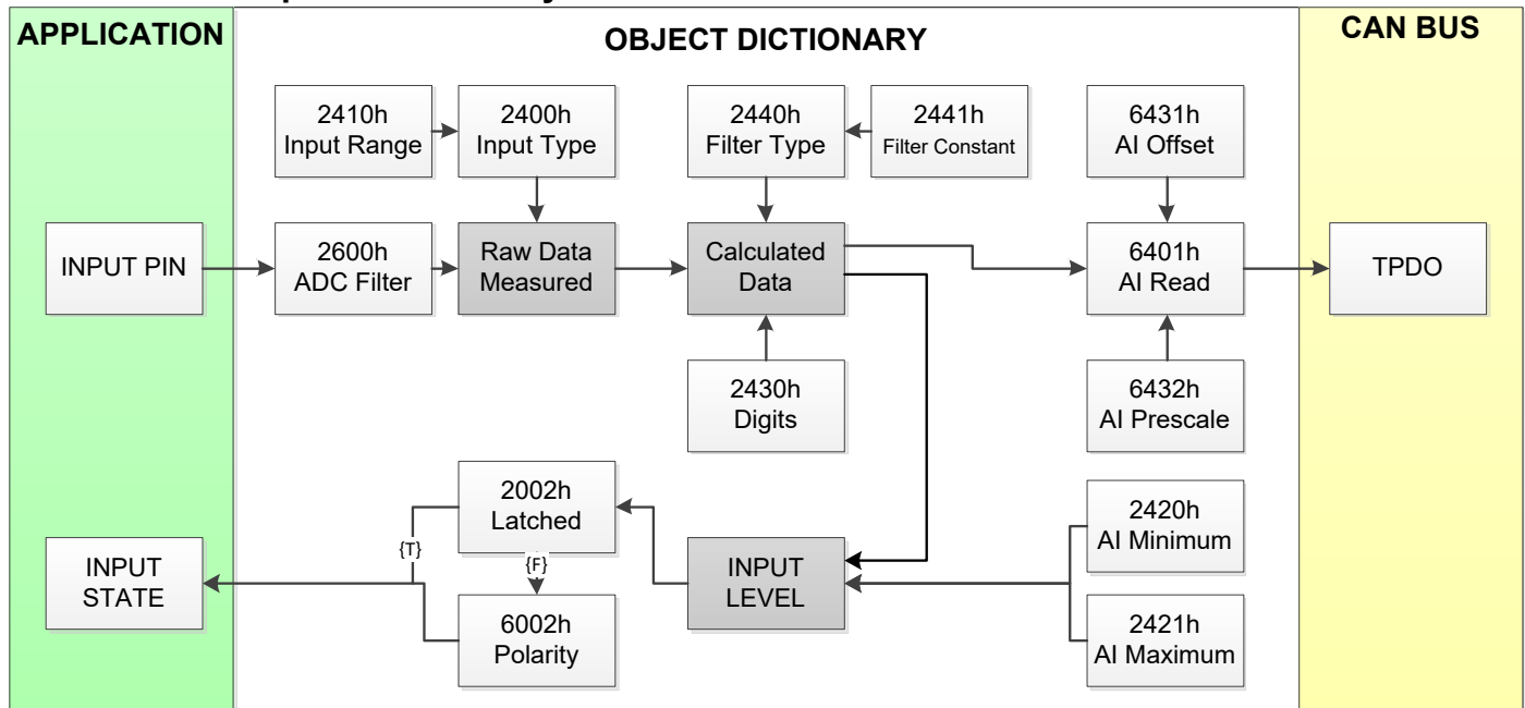
Figure 1 Analog Input Objects
