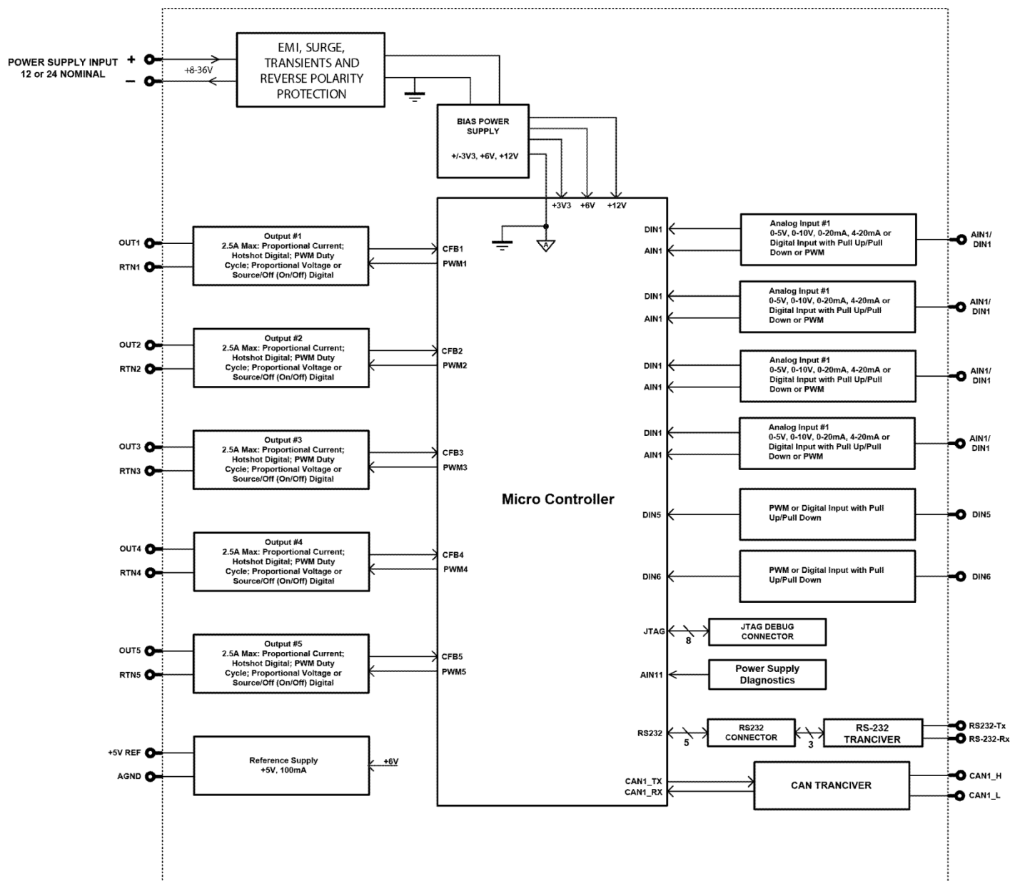
Figure 1 - AX020520 Block Diagram
