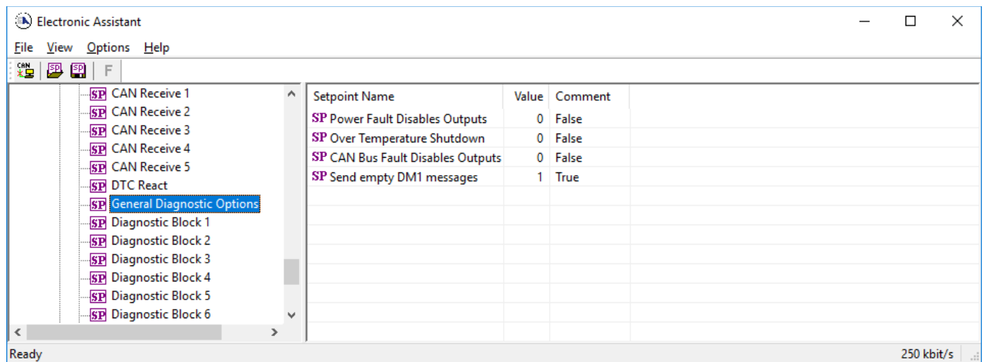
Figure 25 - Screen Capture of General Diagnostics Options Setpoints
