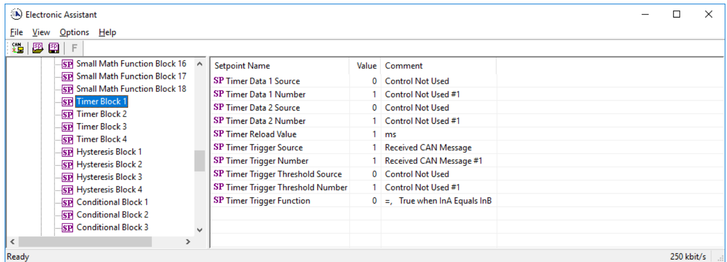
Figure 18 - Screen Capture of Timer Block Setpoints
