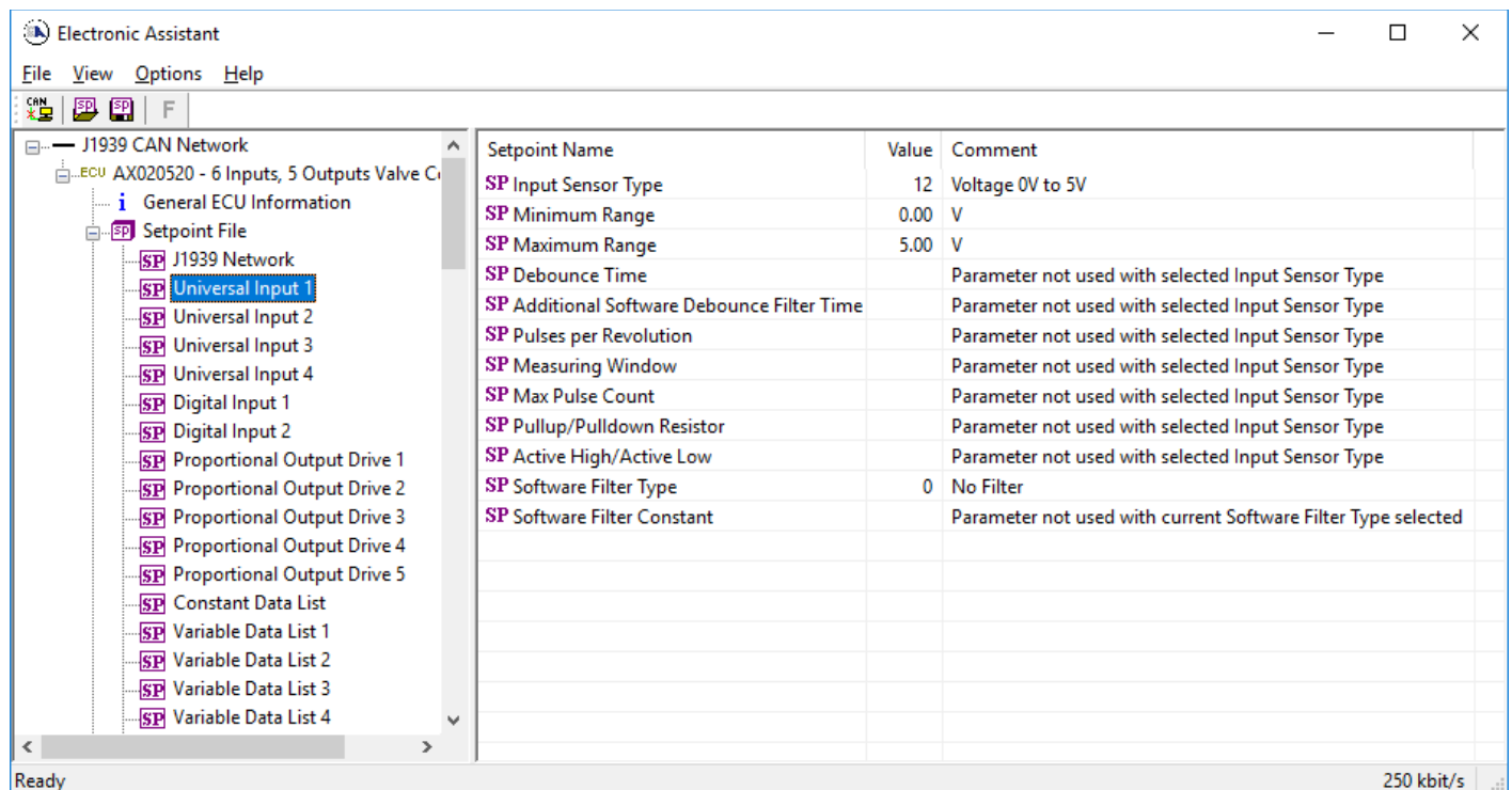
Figure 9 - Screen Capture of Universal Input Setpoints
