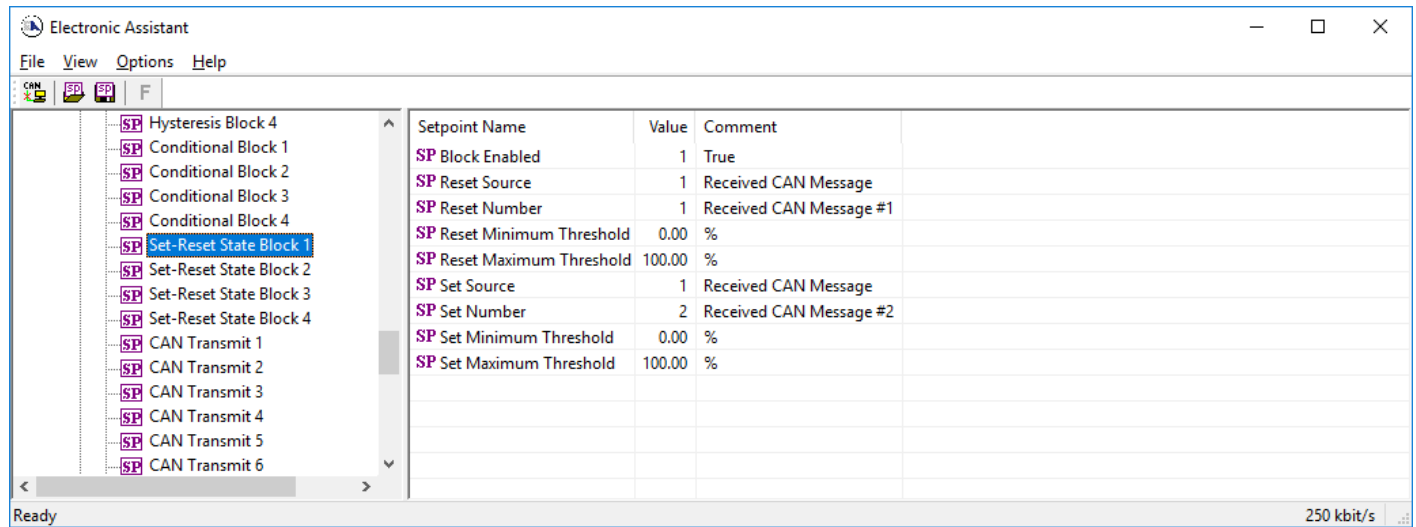
Figure 21 - Screen Capture of Set-Reset State Block Setpoints
