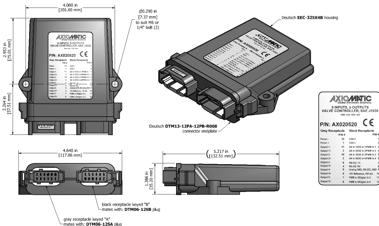
Figure 7 – AX020520 Dimensional Drawing
