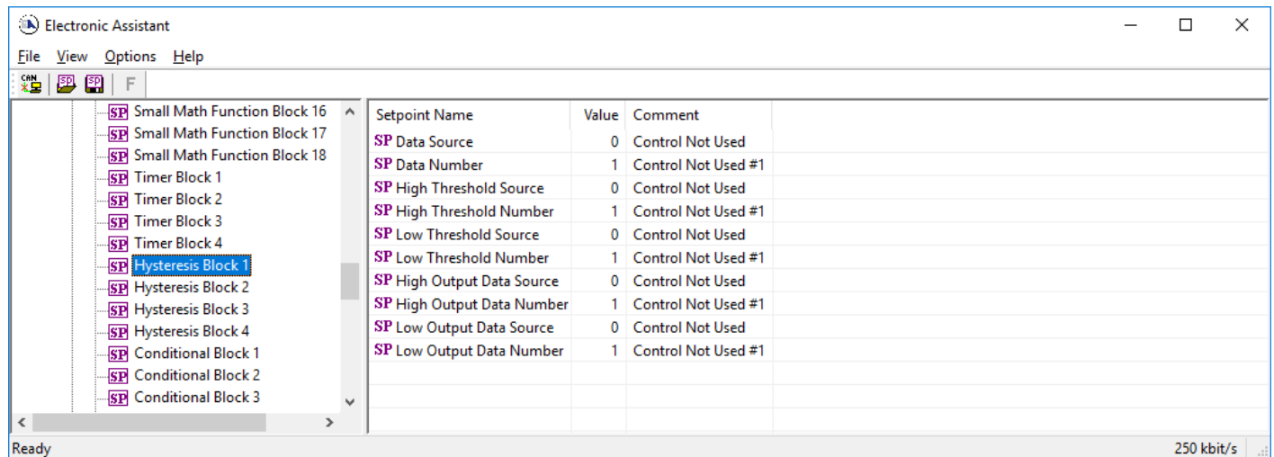
Figure 19 - Screen Capture of Hysteresis Block Setpoints
