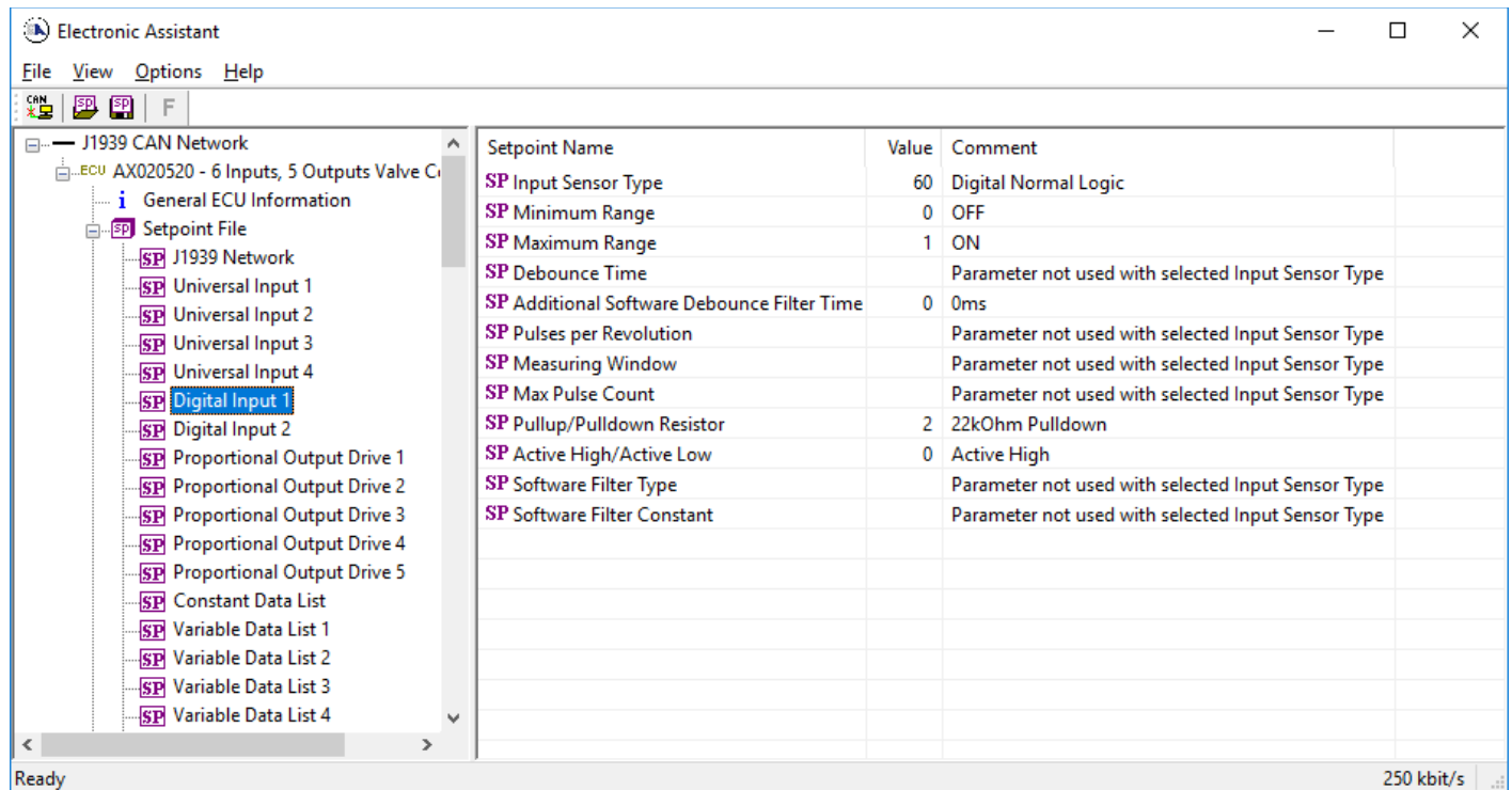
Figure 10 - Screen Capture of Digital Input Setpoints
