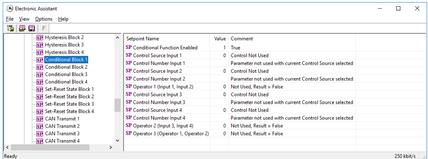
Figure 20 - Screen Capture of Conditional Block Setpoints
