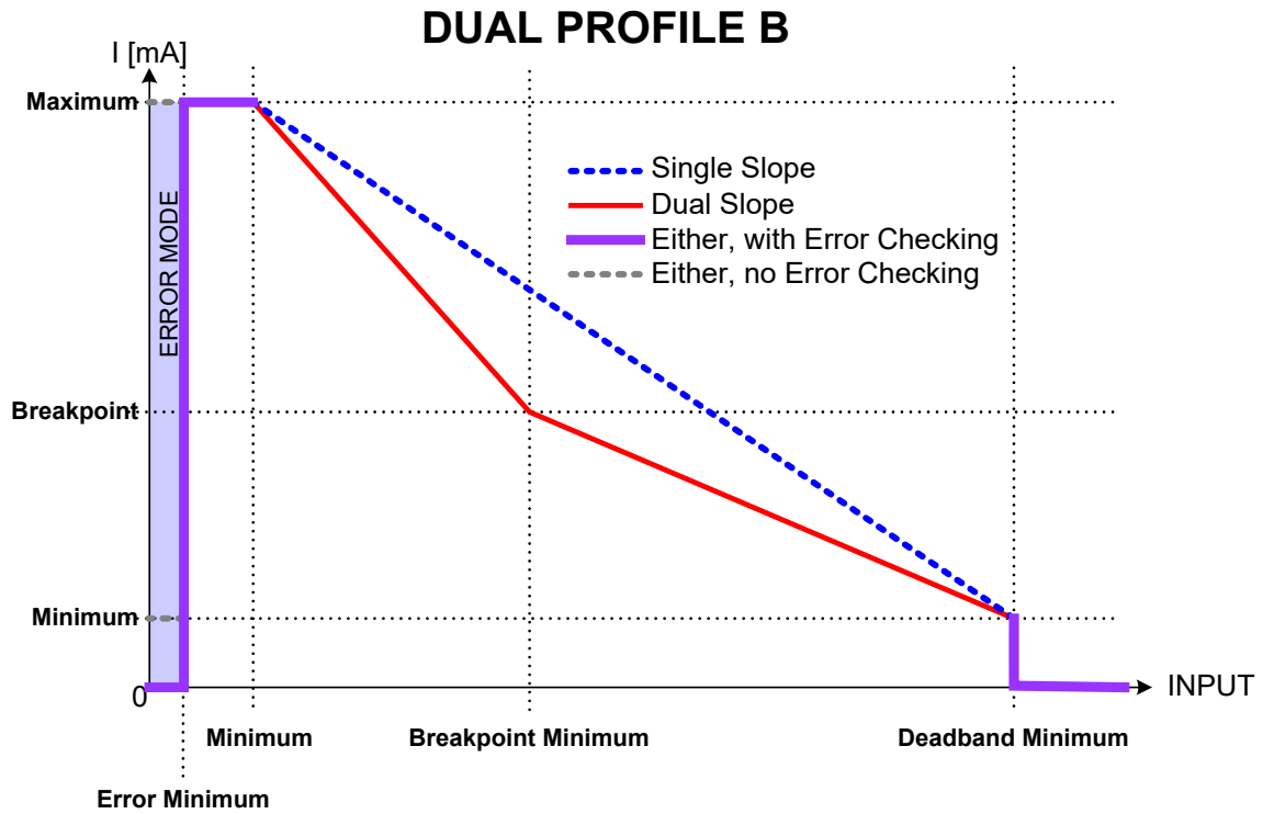
Figure 3 – Proportional Output Dual Profile B
