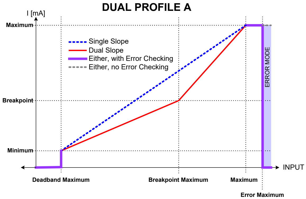
Figure 2 – Proportional Output Dual Profile A
