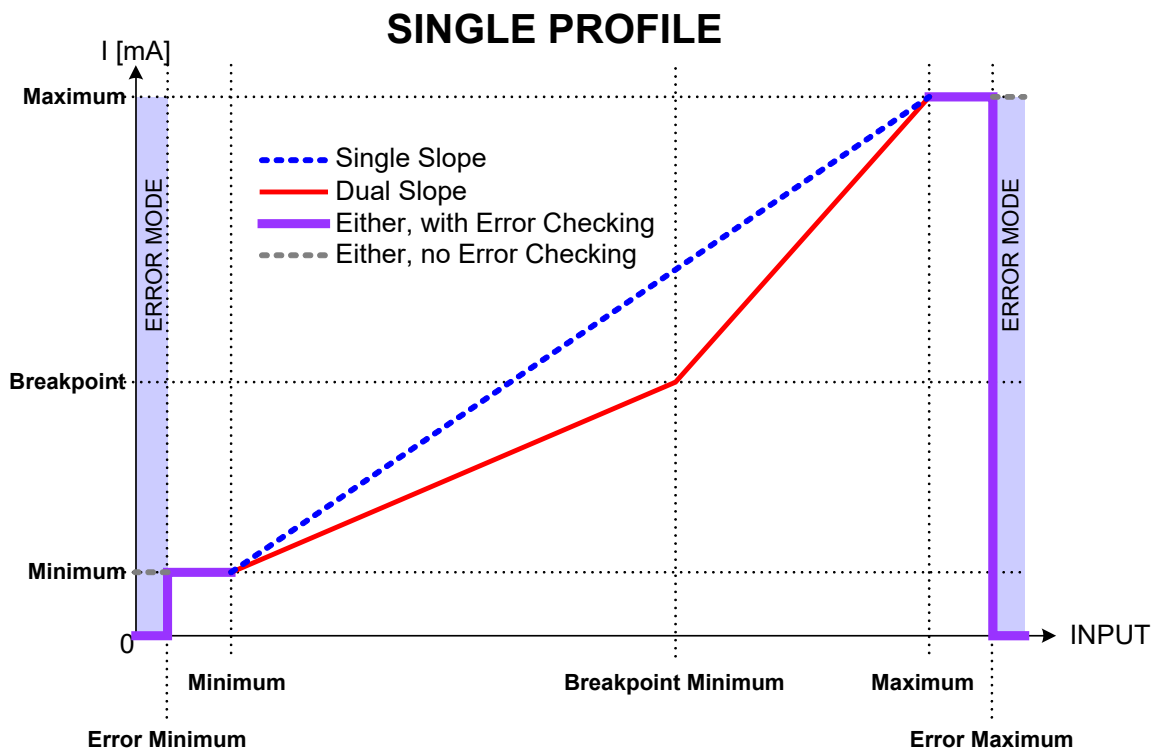
Figure 1 – Proportional Output Single Profile
