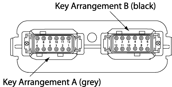
Figure 5 – Housing Diagram
