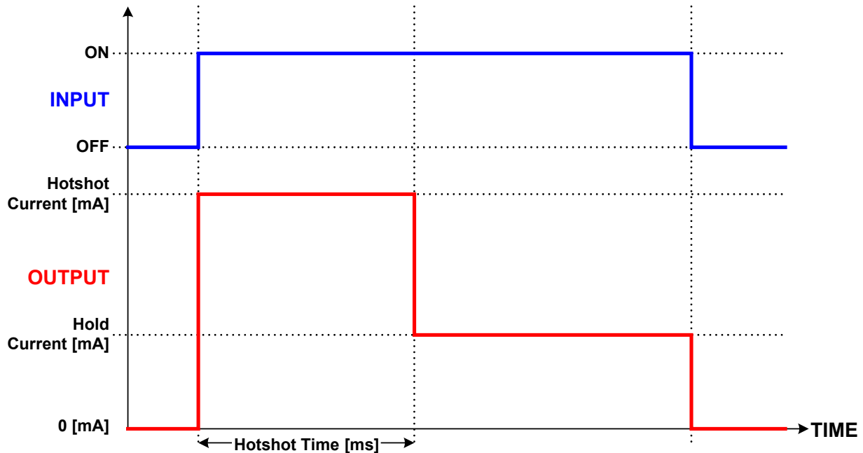
Figure 4 – Proportional Output Hotshot Digital Profile
