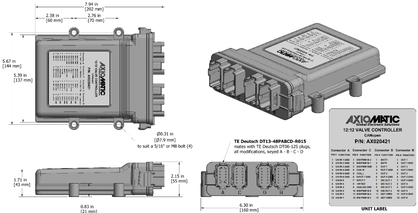
Figure 16 – Housing Dimensions
