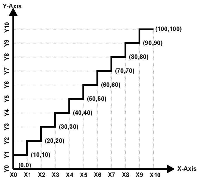
Figure 13 – Lookup Table “Jump To” Data Response
