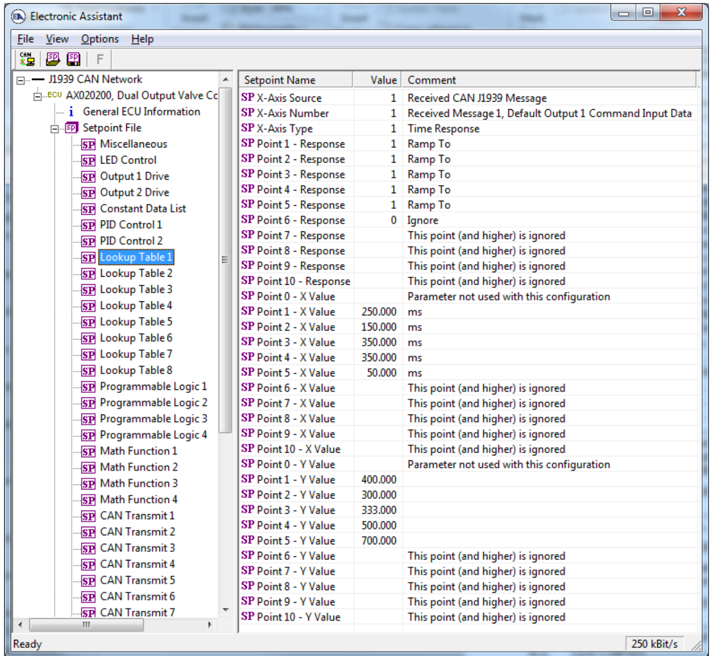
Figure 16 – Lookup Table “Soft Shift” Axiomatic EA Configuration
