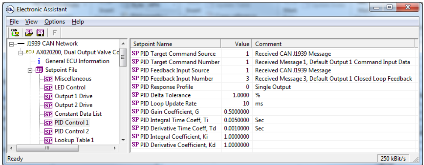
Screen Capture of Default PID Control 1 Setpoints
