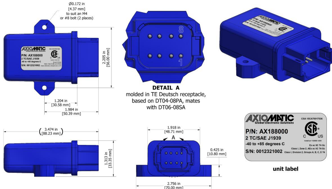
Figure 1.0 - Dimensional Drawing
