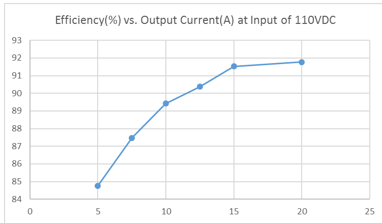
Figure 4.0 - Efficiency vs. Output Current at 110Vdc Input
