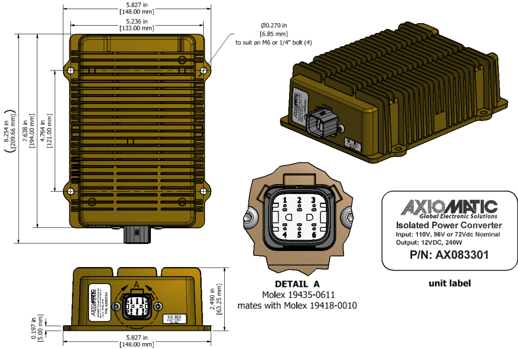
Figure 1.0 – Dimensional Drawing
