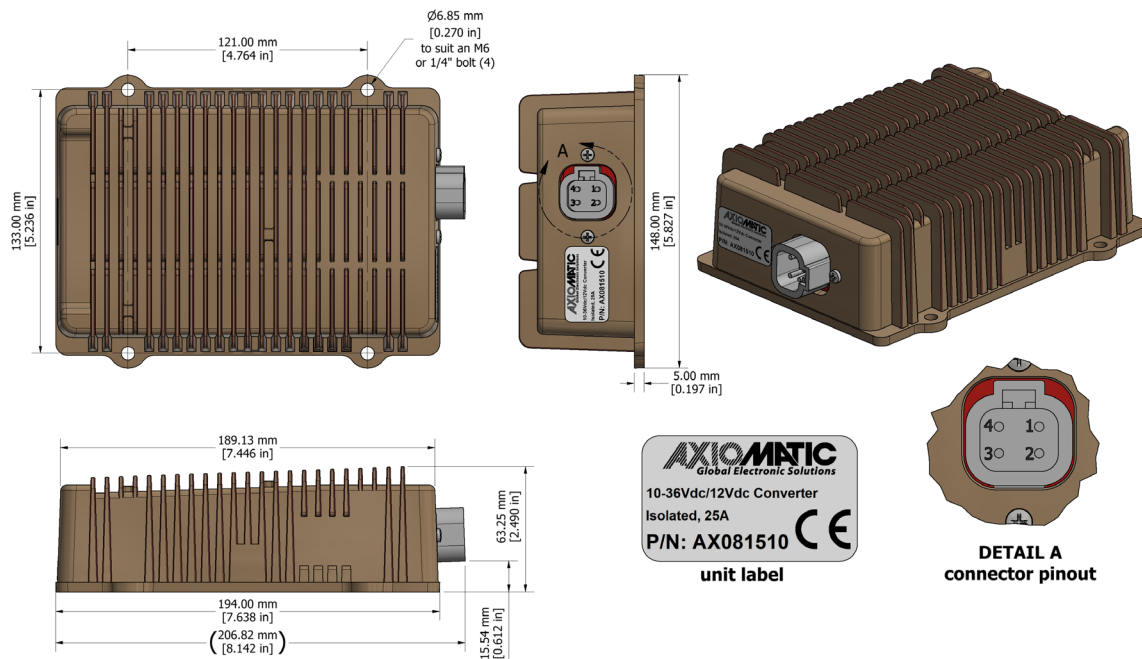
Figure 4. 0. – Dimensional Drawing
