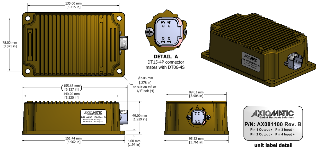
Figure 3.0 – Dimensional Drawing
