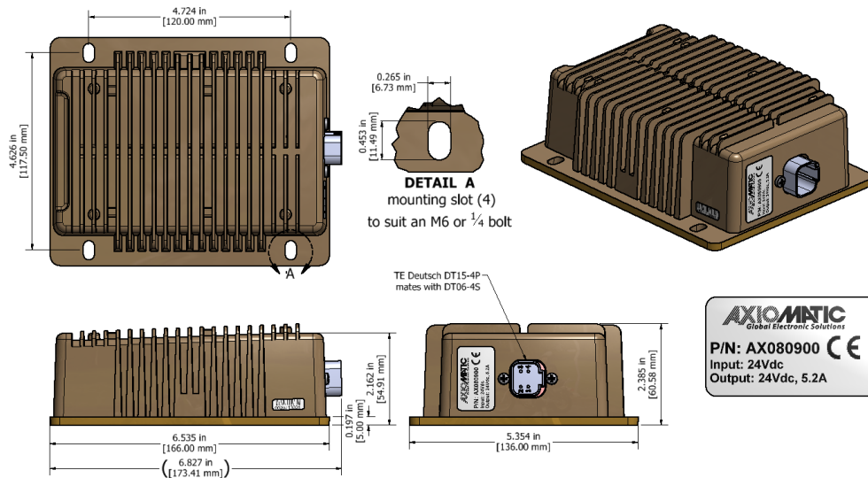
Figure 3.0 – Dimensional Drawing
