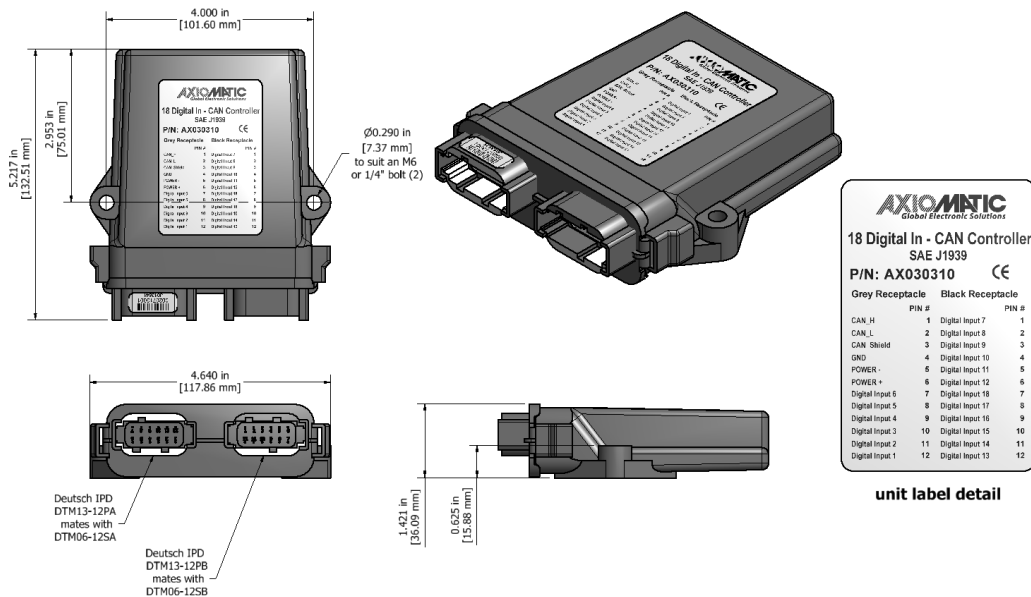
Figure 1.0 - Dimensional Drawing
