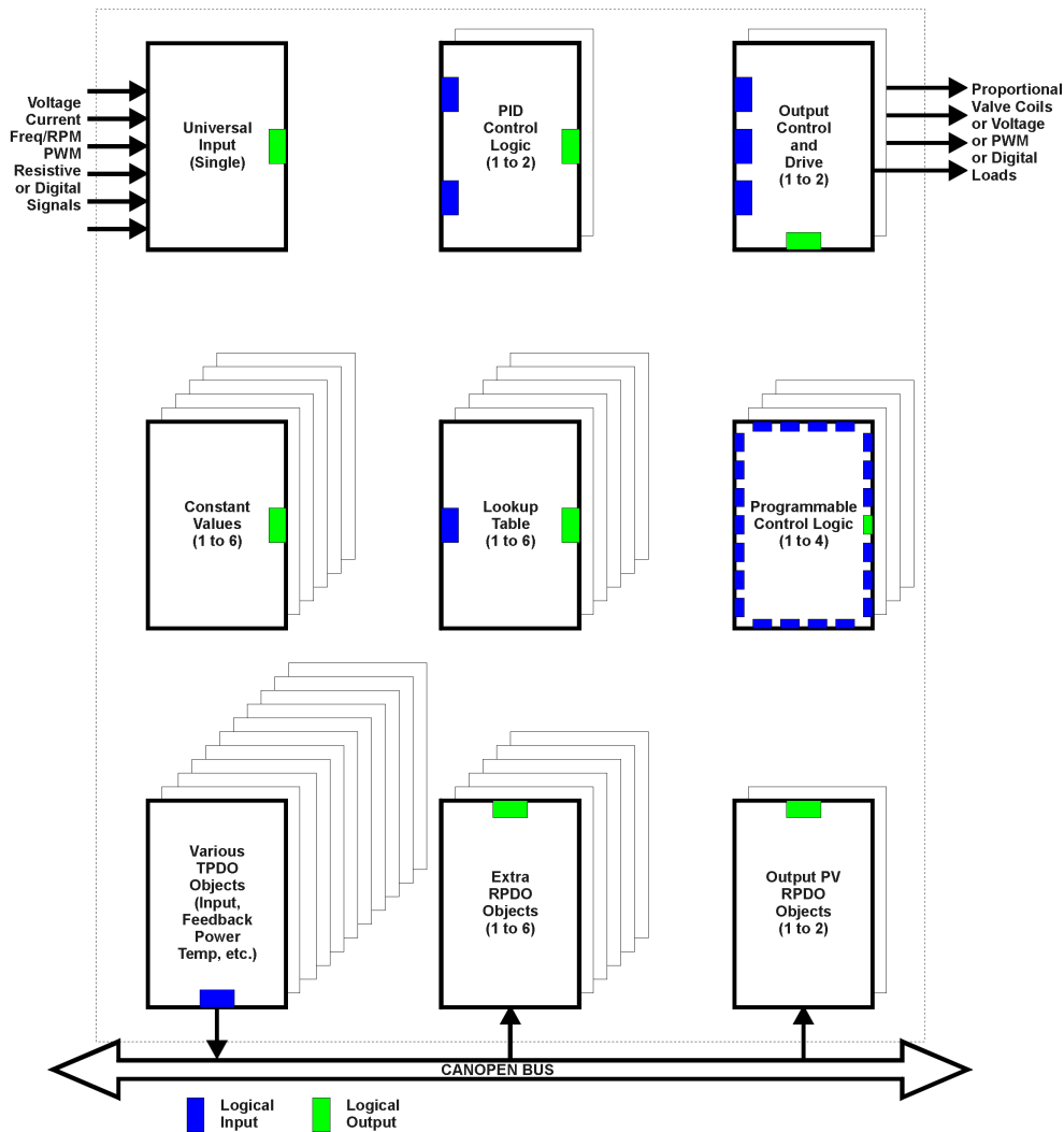
Figure 1 –Logic Functional Block Diagram
