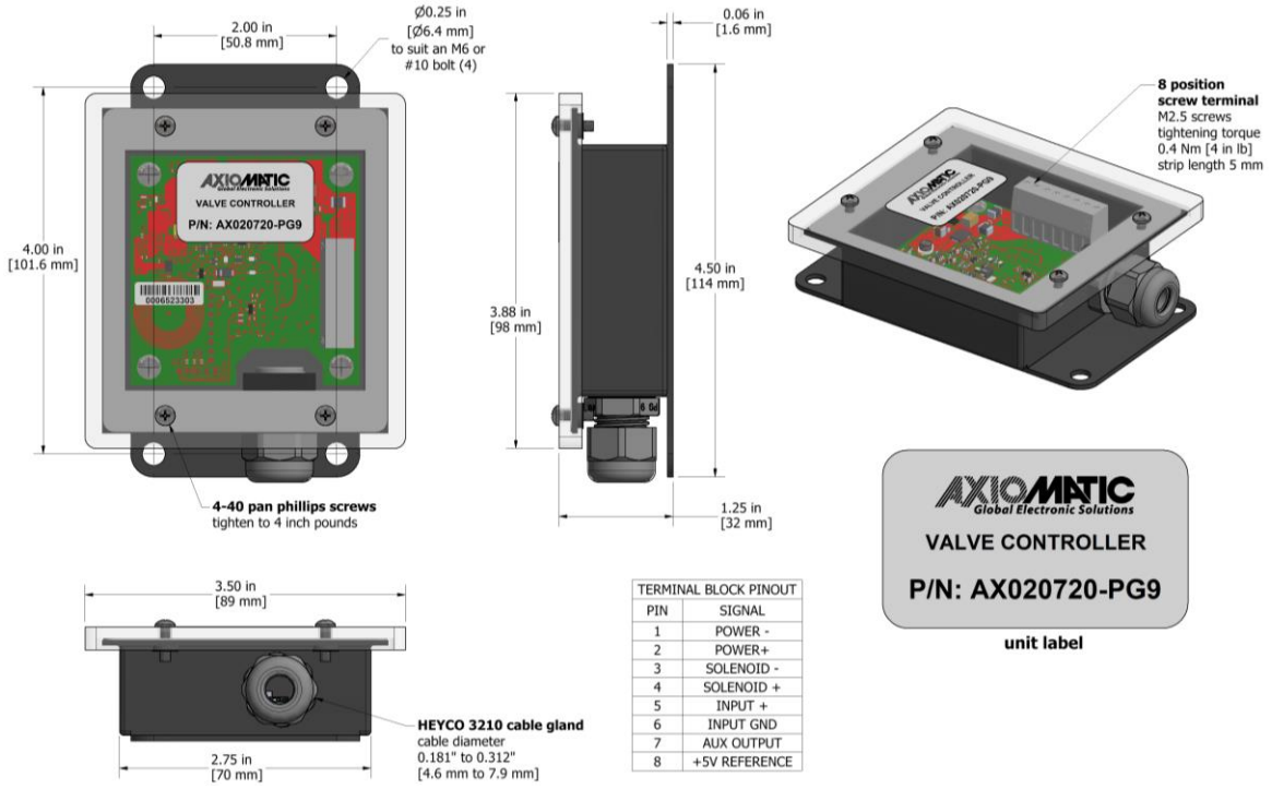
Figure 1.0 – Dimensional Drawing
