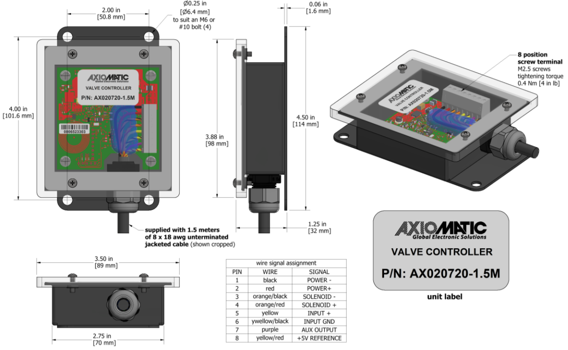
Figure 1.0 – Dimensional Drawing
