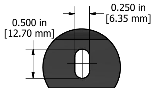
DETAIL A Mounting Slots To Suit M5 Or #12 Bolts
