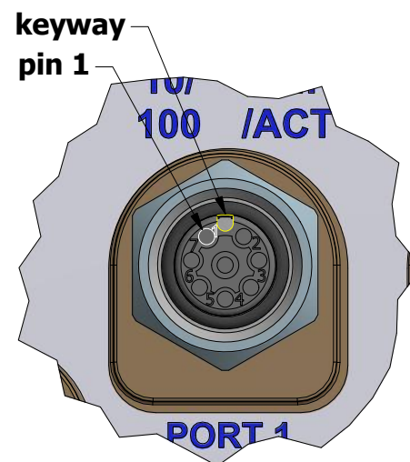
DETAIL A M12 A coded 8 position female
