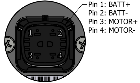
Detail A Molex 19436-0411 4-Pin Connector Mates with Molex 194320001
