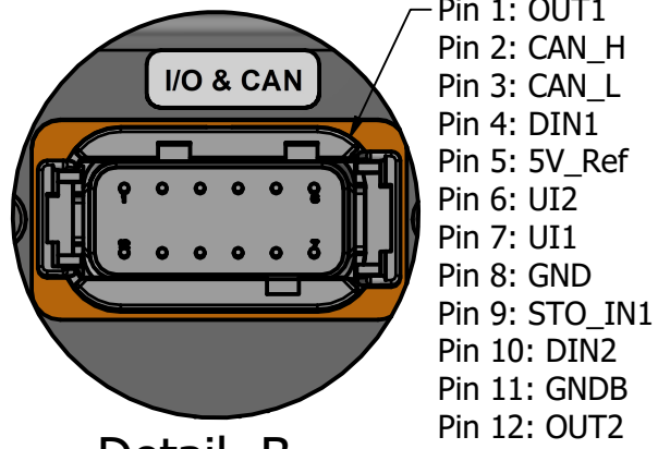
Detail B Deutsch DTM13-12PA 12-Pin Connector Mates with Deutsch DTM06-12SA
