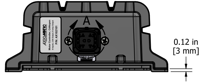
Detail A Molex 19436-0411 4-Pin Connector Mates with Molex 194320001
