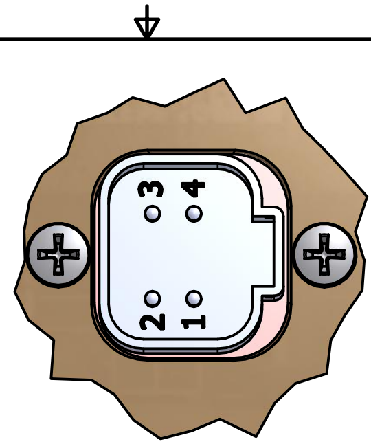
DETAIL A DT15-4P connector mates with DT06-4S
