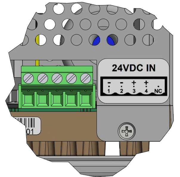
DETAIL B input connector pluggable terminal blocks with screw terminal connections, 5.08 mm [0.200"] pitch
