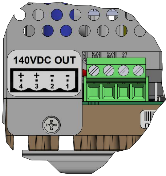
DETAIL A output connector pluggable terminal blocks with screw terminal connections, 5.08 mm [0.200"] pitch
