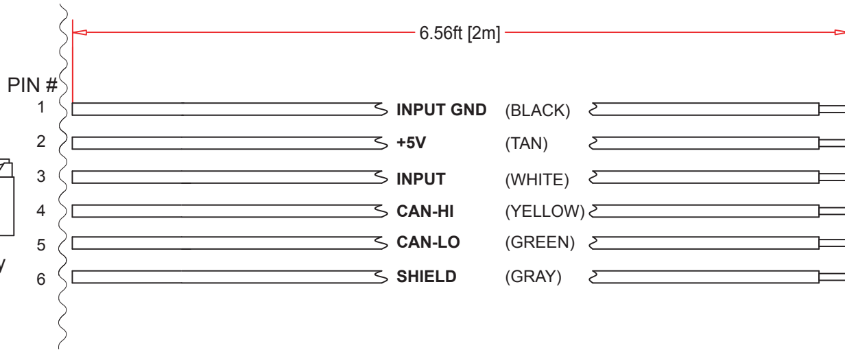
DT06-6S Assembly
