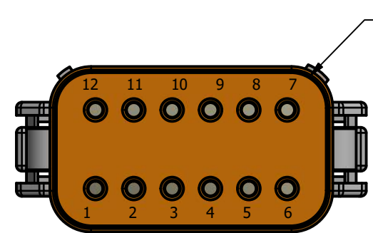
Detail A Deutsch DT06-12SA 12-Pin Plug Mates With DT13-12PA Connector
