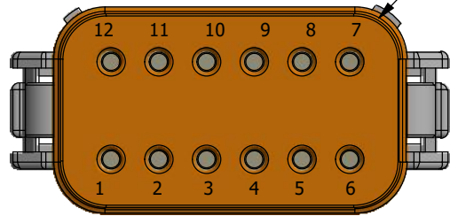
Detail A Deutsch DT06-12SA 12-Pin Plug Mates With DT13-12PA Connector
