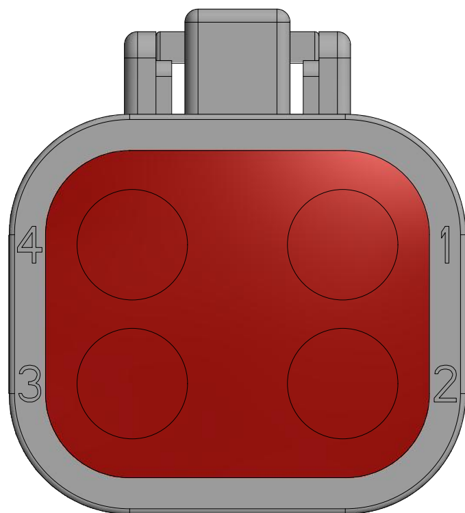
DTP06-4S pinout
