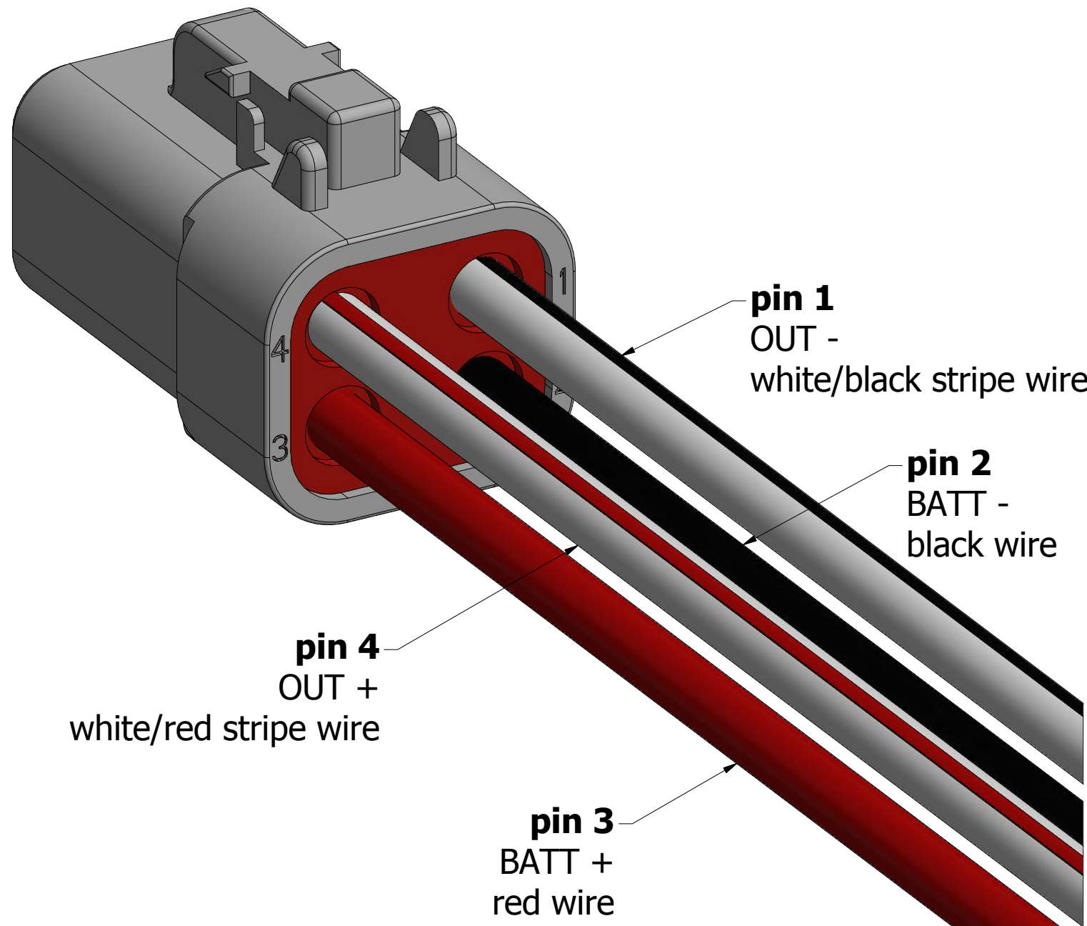
2 meter long power connector cable assembly for use with AX100310 motor controller
