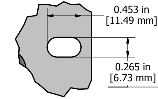
DETAIL A mounting slots
