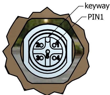
DETAIL B 5 pin A coded M12 male input connector
