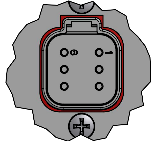
DETAIL A TE Deutsch DT15-6P mates with DT06-6S
