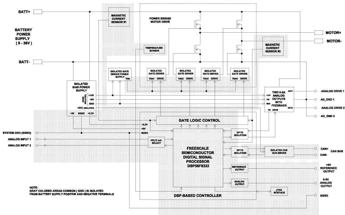
Block Diagram
